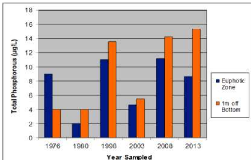
KASHWAKAMAK LAKE - ALL BASINS ANNUAL MEAN TOTAL PHOSPHORUS RESULTS (ug/L)
