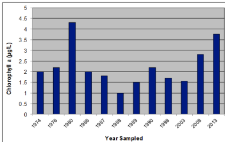
KASHWAKAMAK LAKE - ALL BASINS ANNUAL MEAN CHLOROPHYLL a RESULTS (ug/L)
