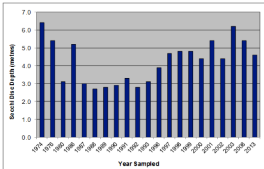
KASHWAKAMAK LAKE — ALL BASINS ANNUAL MEAN SECCHI DISC DEPTHS (metres)
