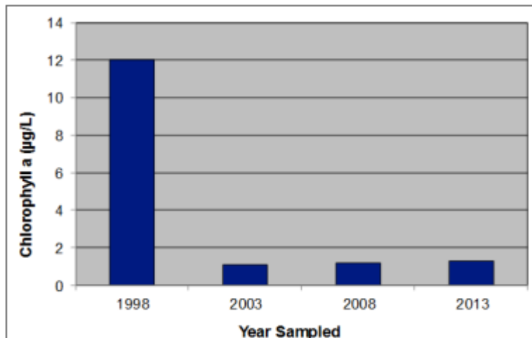
MCCAUSLAND LAKE - MAIN BASIN ANNUAL MEAN CHLOROPHYLL a RESULTS (ug/L)
