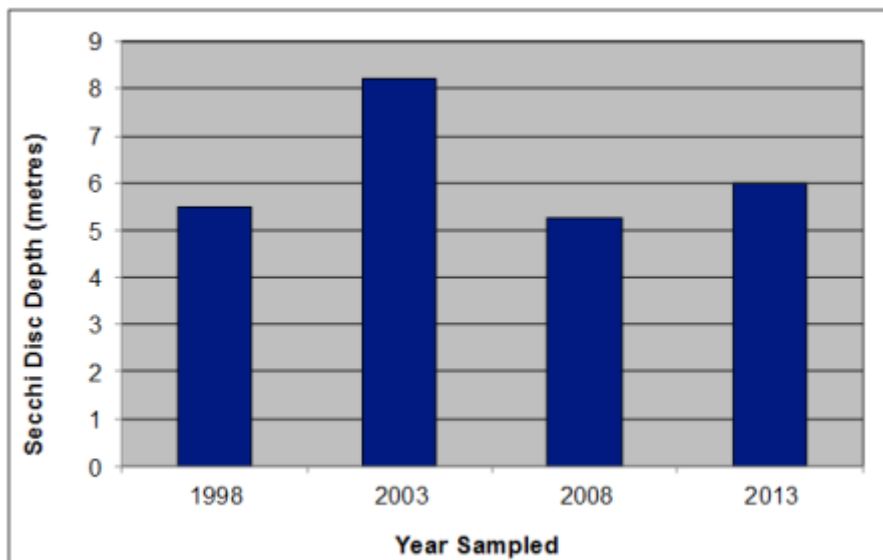
MCCAUSLAND LAKE — MAIN BASIN ANNUAL MEAN SECCHI DISC DEPTHS (metres)
