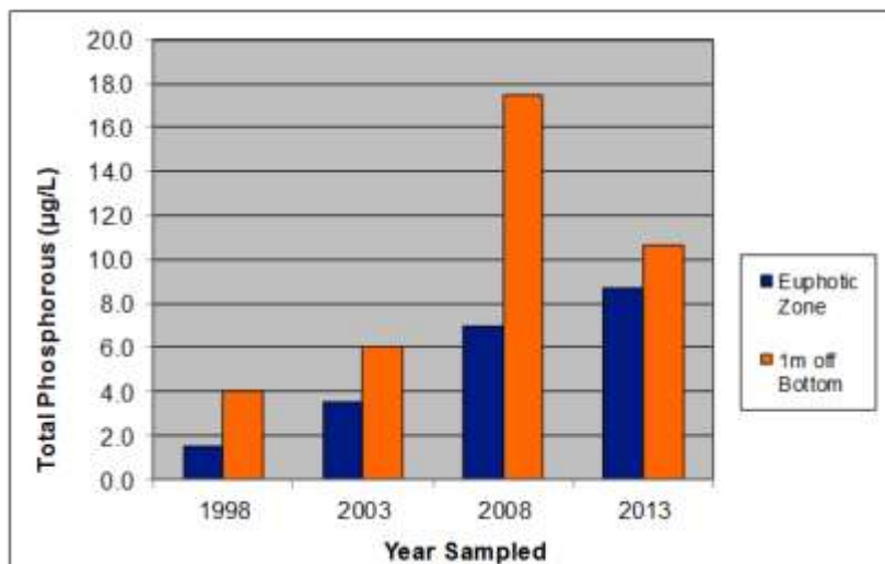
MCCAUSLAND LAKE - MAIN BASIN ANNUAL MEAN TOTAL PHOSPHORUS RESULTS (ug/L)
