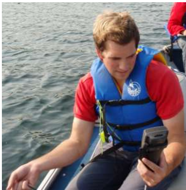
The Dissolved Oxygen Metre is used to gather DO and temperature readings. The probe is lowered into the lake and readings are taken at every metre from the hand-held screen.
